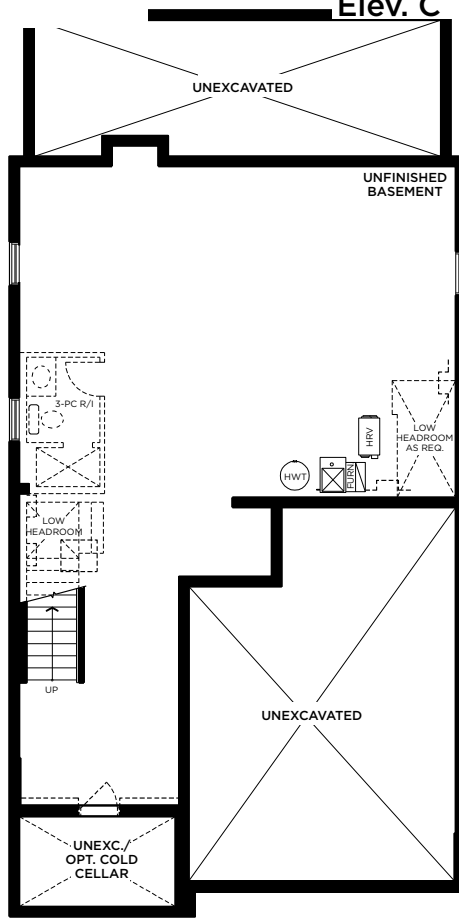
BASEMENT PLAN Elev. A
